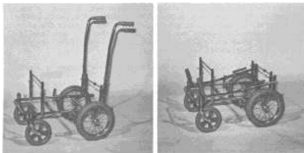
A special castored base is also custom made to accommodate the fiberglass seat support for manual propulsion by an attendant. The push handles of the castored base may be released and folded down for storage in vehicles.
